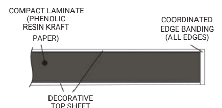
COMPACT LAMINATE CROSS SECTION
