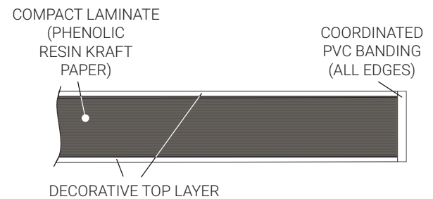
COMPACT LAMINATE CROSS SECTION
