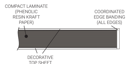
COMPACT LAMINATE CROSS SECTION
