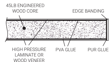
HIGH PRESSURE LAMINATE AND WOOD VENEER CROSS SECTION
